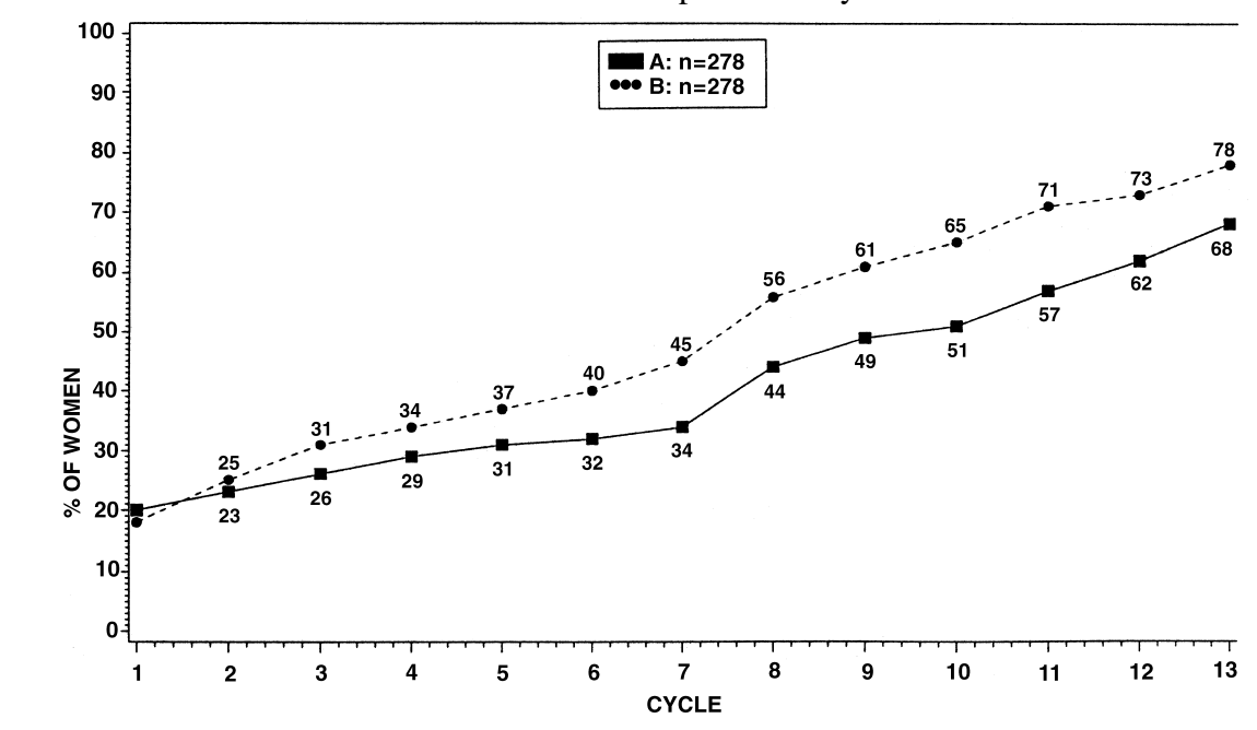
Figure 2. Patients with Cumulative Amenorrhea Over Time (Percentage of Women With No Bleeding or Spotting at a Given Cycle Through Cycle 13) All Patients Who Completed 13 Cycles
